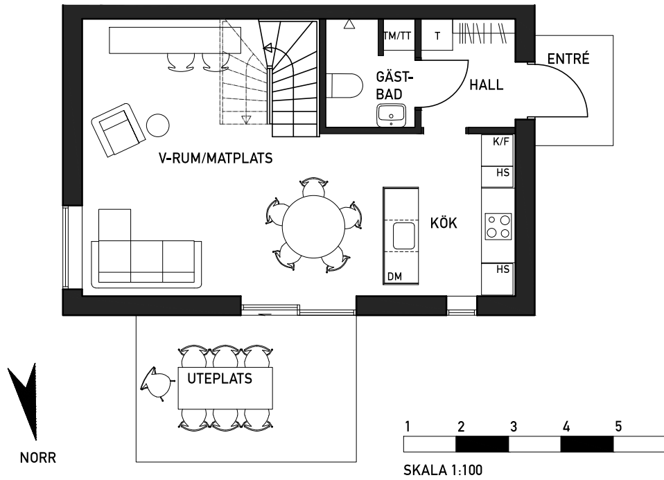
HUS 1D PLAN 1
